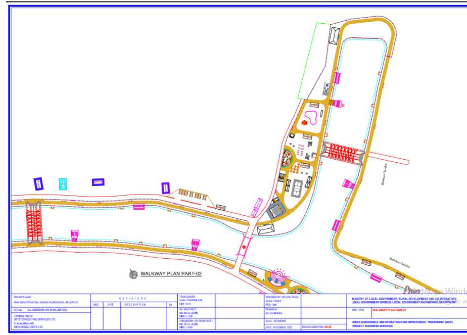
Figure-1: Proposed Site Plan Lake Beautification
